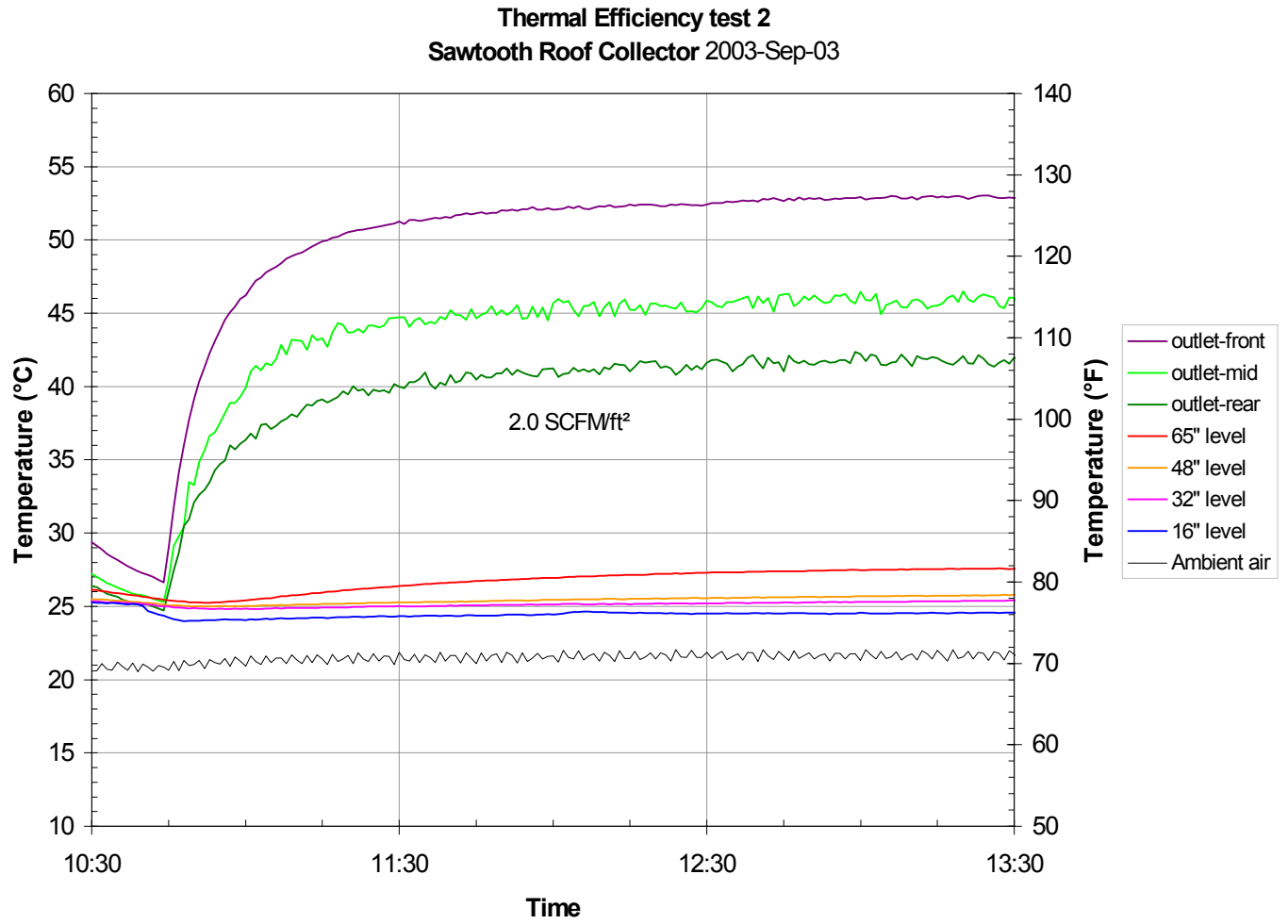
Figure 3. Air temperatures recorded during second thermal efficiency test.
